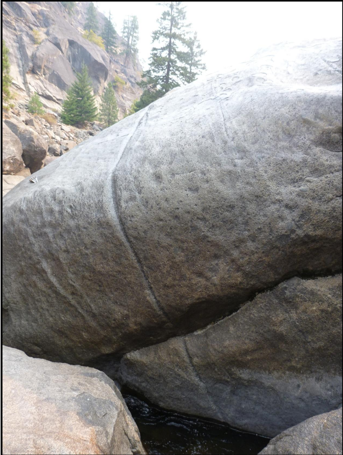
Figure 9. A vertical glacial groove and horizontal discontinuity on the upstream face of Anchor Boulder.
